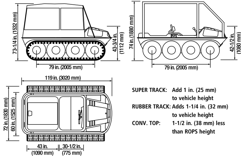
Vehicle shown with accessories, see specification page for base vehicle. (ARGO 8x8 750 HDI model shown)
